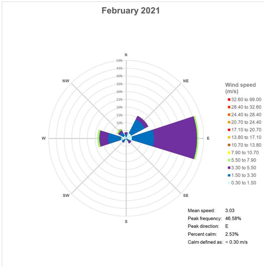
Figure 1. Wind rose data – February 2021
