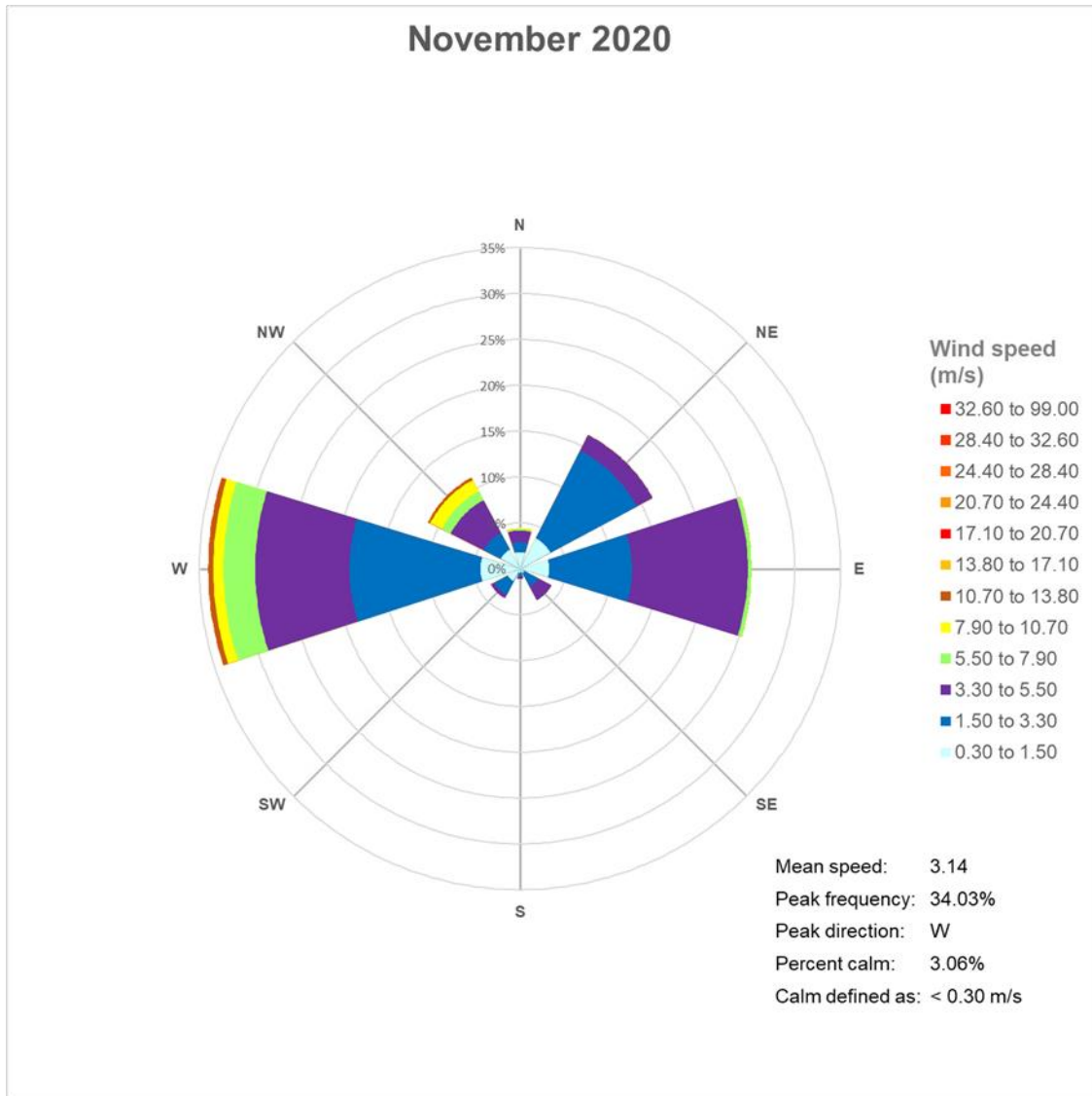
Figure 1. Wind rose data – November 2020
