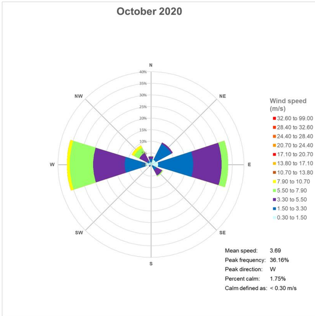
Figure 1. Wind rose data – October 2020
