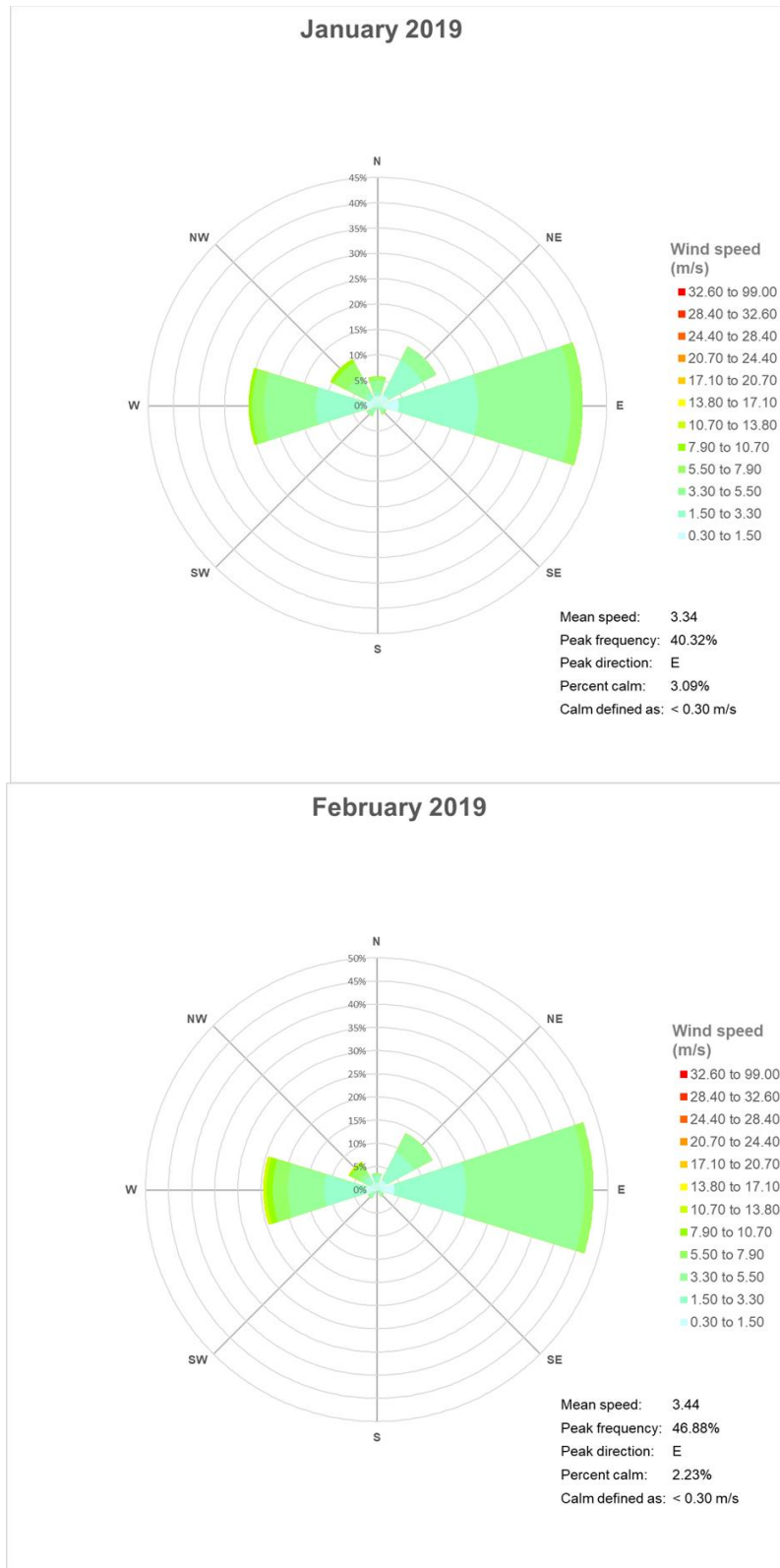
Figure 1. Prevailing wind direction (percentage for month) December 2018 - February 2019
