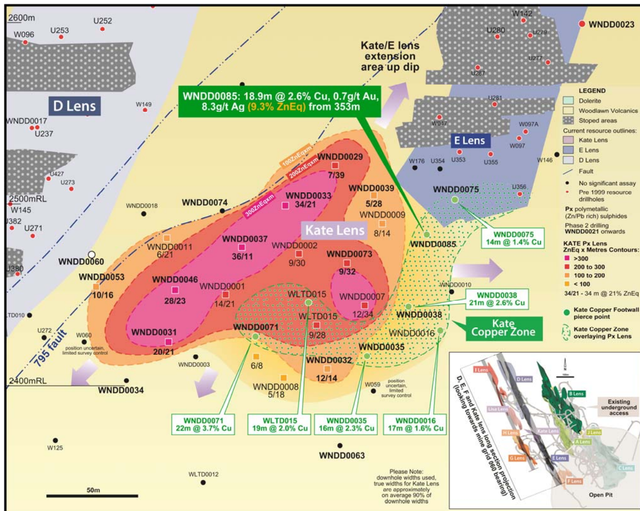
Figure 1: Kate Lens Long-Section looking east with recent Kate Copper intercepts shown. Down-hole intercept thickness and ZnEq grade contoured to show relative accumulation of metals across the lens.
