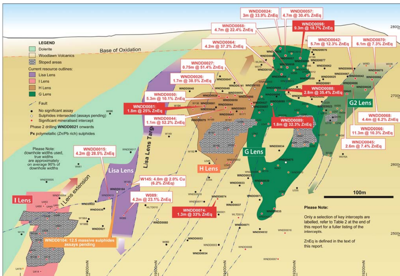
Figure 2: Lisa, G, H, E Lenses Long-Section looking east with recent intercepts shown.
