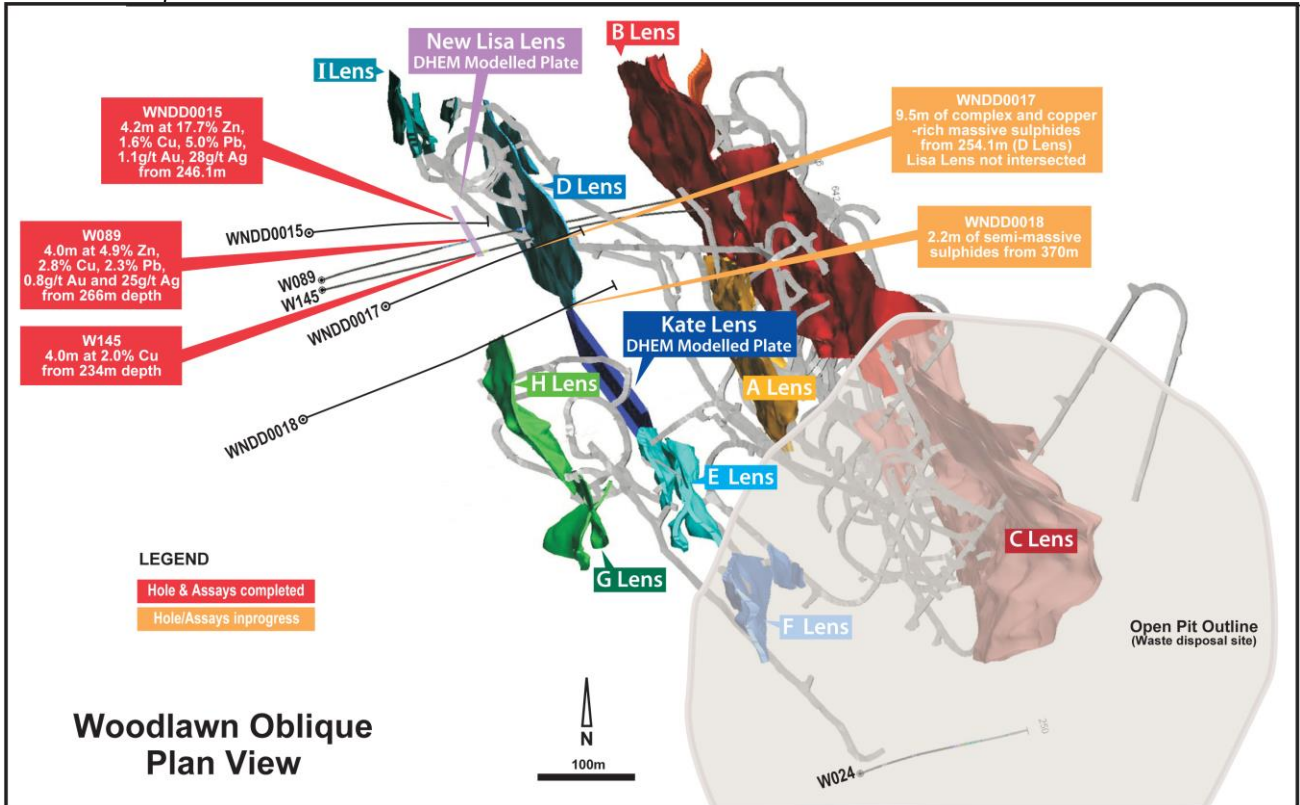
Figure 1: Plan overview of the Woodlawn Lenses showing pit and existing underground decline. The new Lisa Lens is shown in the top left hand corner.
