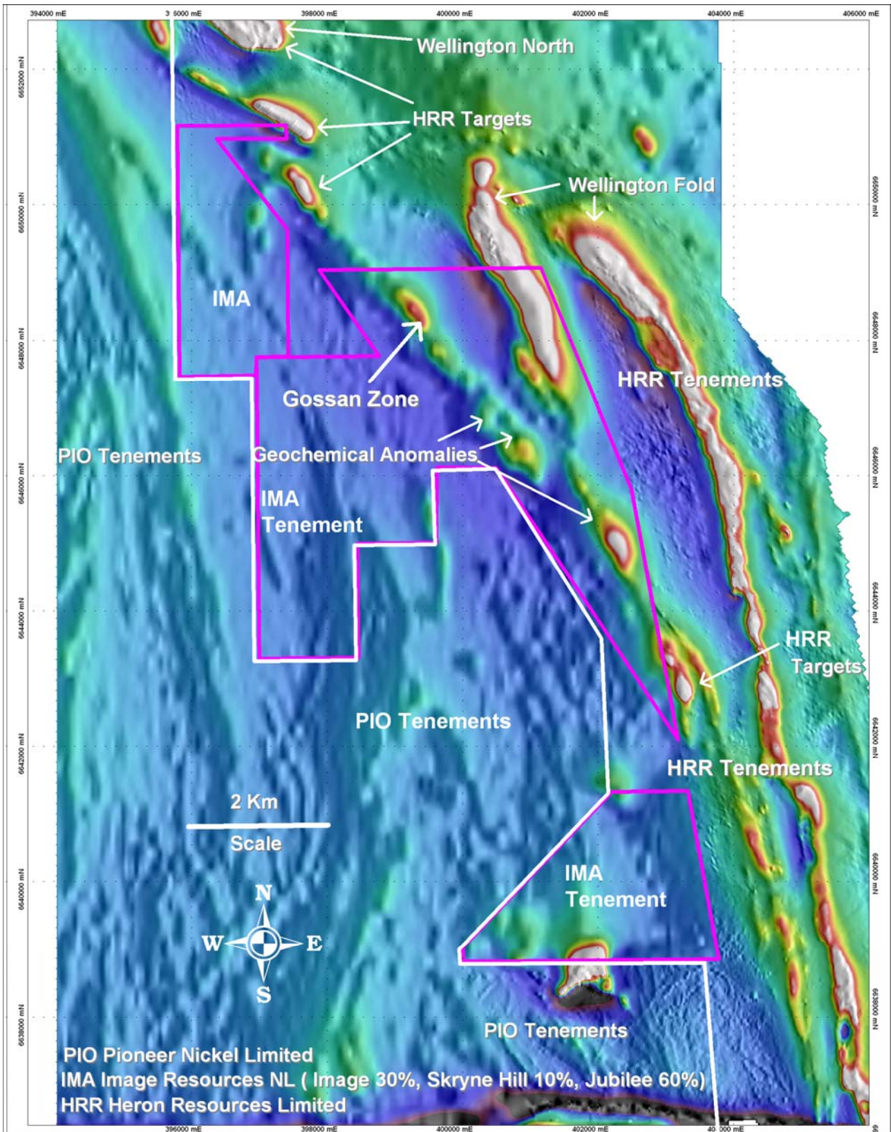
Figure 1 Total Magnetic Intensity and Tenement Holdings, Emu Lake-Kalpini area
